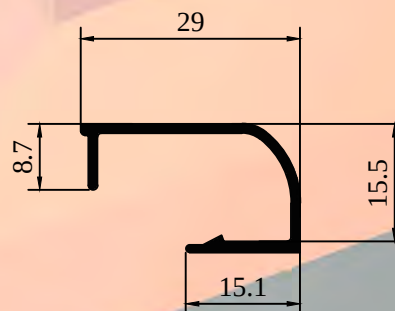
ALX-2230 CONTRAVIDRIO 29mm
